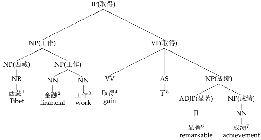
Figure 5 A syntactic parse tree with head word annotated for each internal node. The superscripts of leaf nodes denote their surface positions from left to right.
